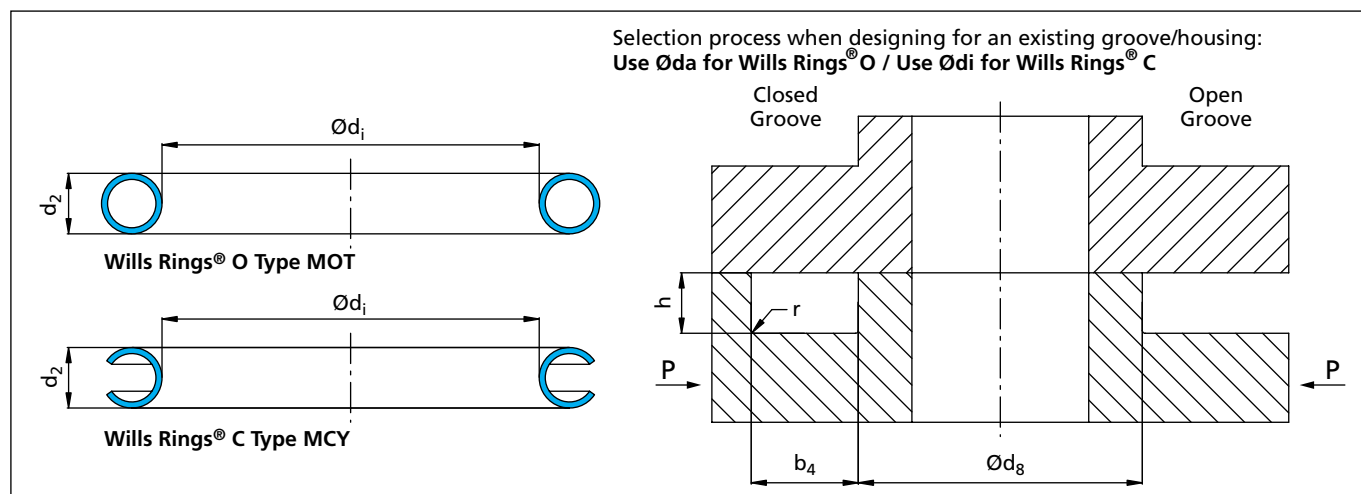
Figure 17 Installation drawing for external pressure
