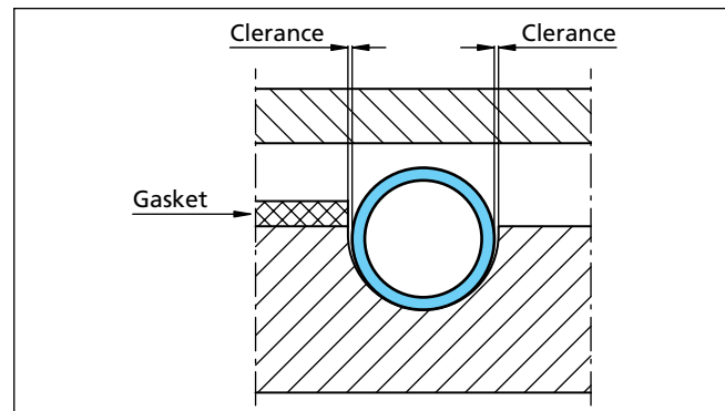
Figure 14 Detail of an automotive groove
