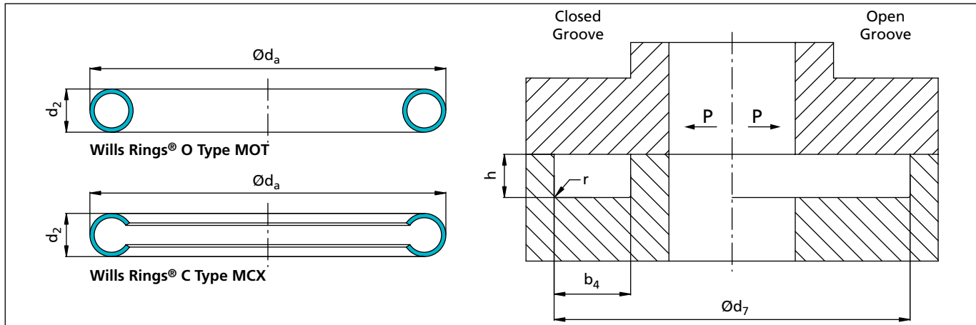
Figure 16 Installation drawing for internal pressure
