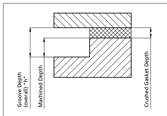
Figure 15 Wills Rings® groove depth with a gasket
