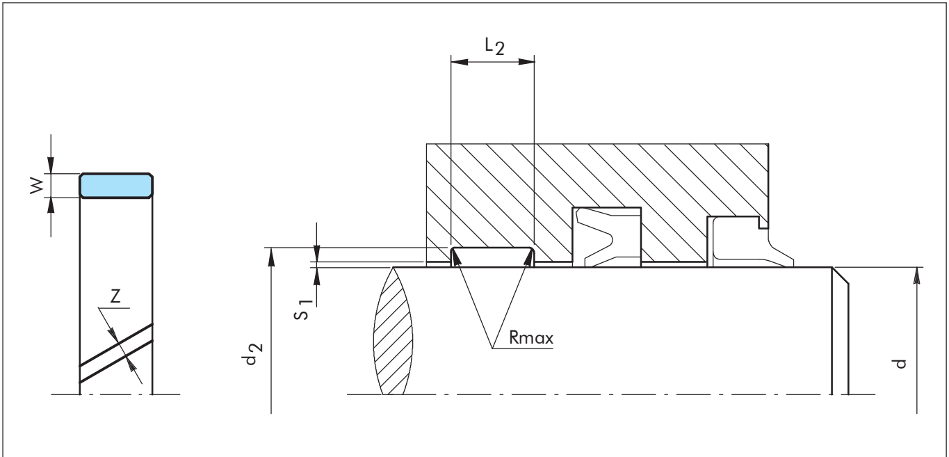
Figure 24 Installation drawing
