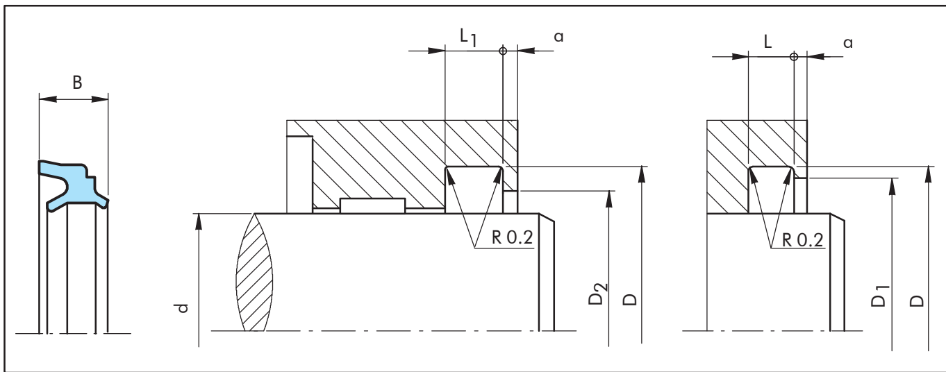
Figure 14 Installation Drawing
