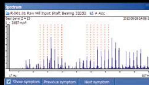
Spectrum with gear symptom
