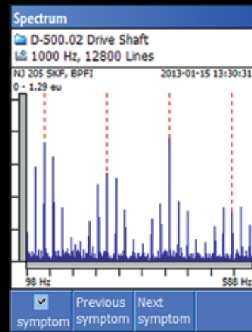
Vibration spectrum from an EVAM measurement
