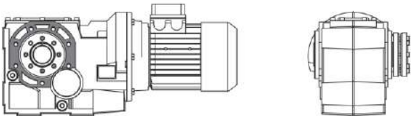
SL FLANGE MOUNTING / HOLLOW SHAFT
